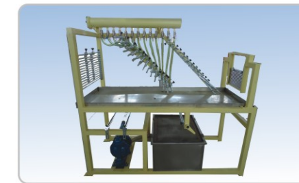
D 型上胶架 (D gluing system)
